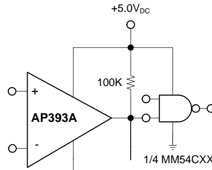
Driving CMOS
