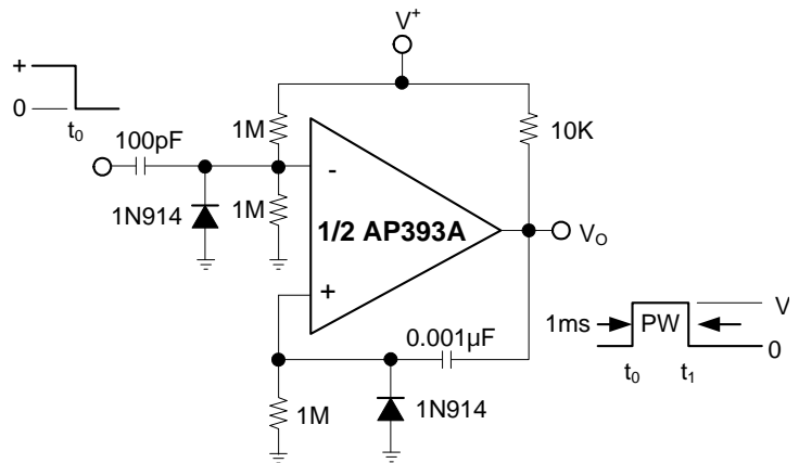
One-Shot Multivibrator
