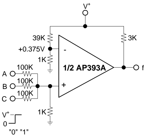
AND Gate
