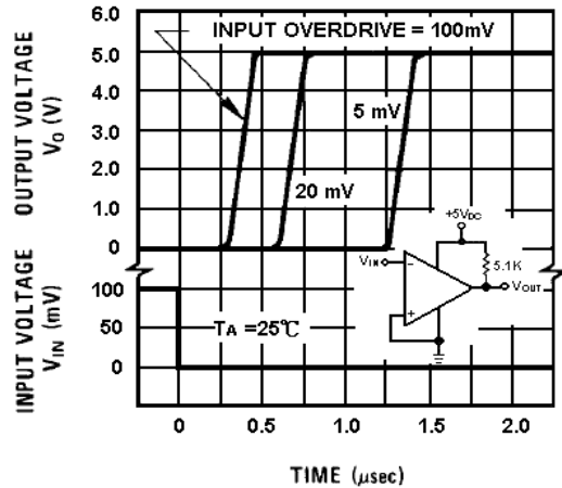
Response Time for Various Input Overdrives—Positive Transition
