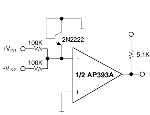
Comparing Input Voltages of Opposite Polarity
