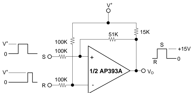
Bi-Stable Multivibrator
