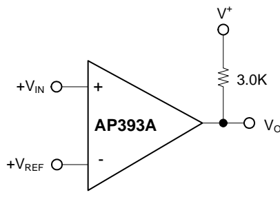
Basic Comparator
