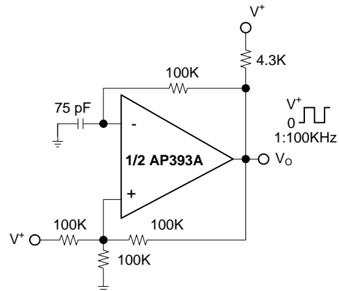
Squarewave Oscillator
